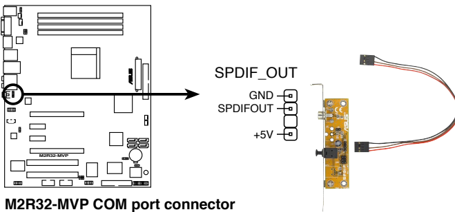
M2R32-MVP COM port connector
