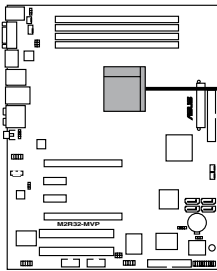
M2R32-MVP CPU Socket AM2
