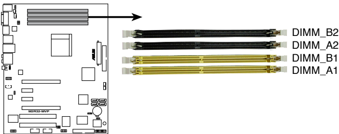
M2R32-MVP 240-pin DDR2 DIMM sockets
