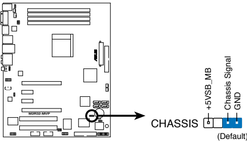
M2R32-MVP Chassis intrusion connector
