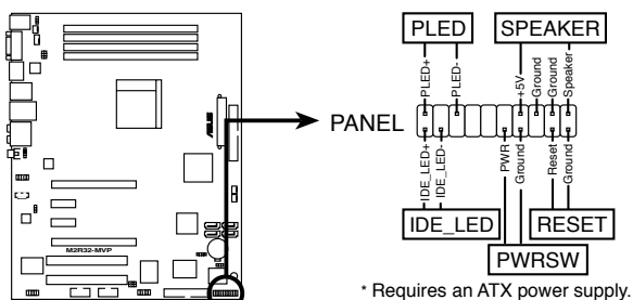
M2R32-MVP System panel connector
