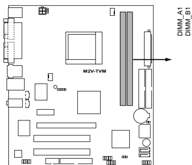
M2V-TVM 240-pin DDR2 DIMM Sockets
