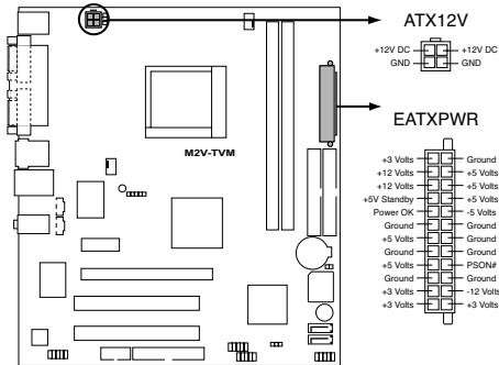
M2V-TVM ATX power connectors
