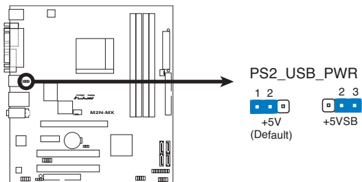
USB device wake-up de la M2N-MX
