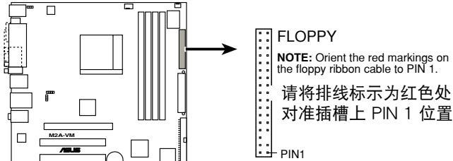
M2A-VM Floppy disk drive connector
