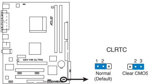
A8V-VM ULTRA Clear RTC RAM
