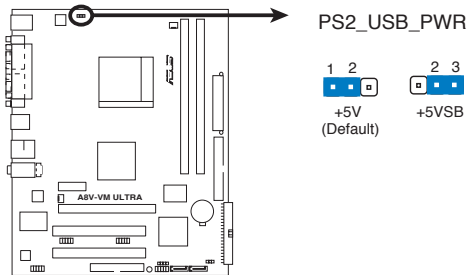
A8V-VM ULTRA USB Device Wake Up
