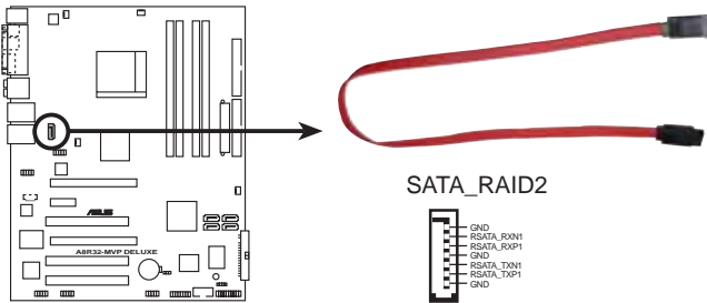
A8R32-MVP DELUXE SATA RAID connector
