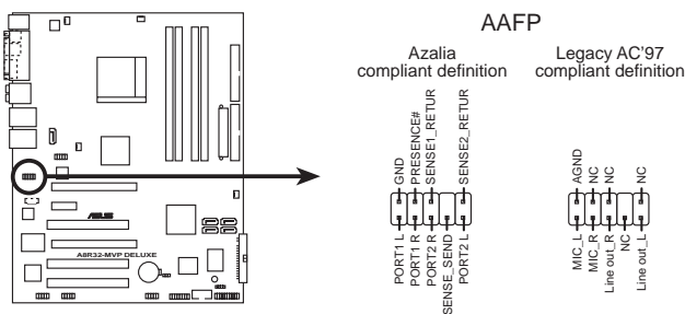
A8R32-MVP DELUXE Analog front panel connector
