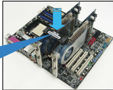
Conector SLI
