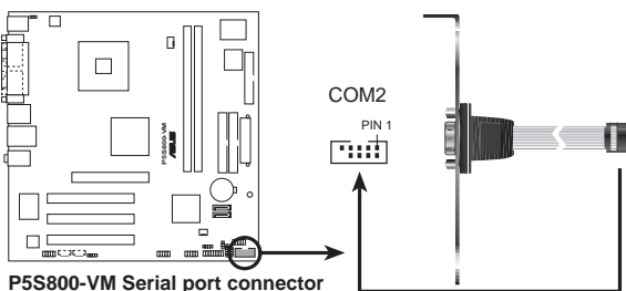
P5S800-VM Serial port connector
