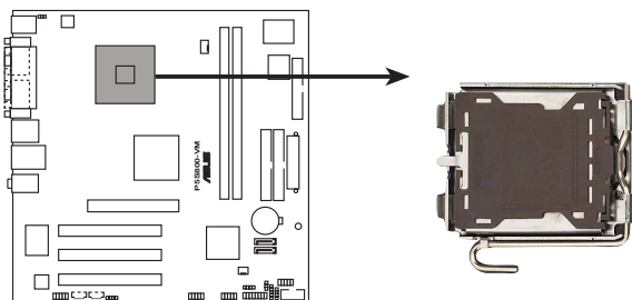
P5S800-VM CPU Socket 775
