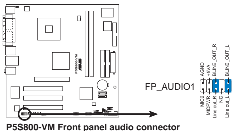
P5S800-VM Front panel audio connector
