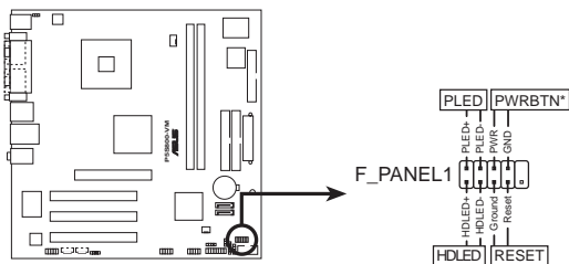
P5S800-VM System panel connector
