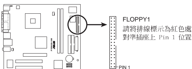
P5S800-VM Floppy disk drive connector
