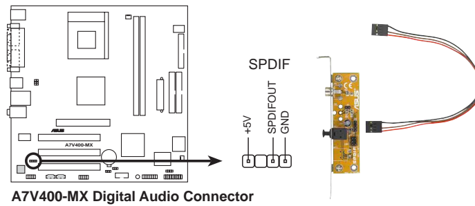
A7V400-MX Digital Audio Connector
