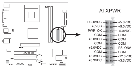
A7V400-MX ATX Power Connector
