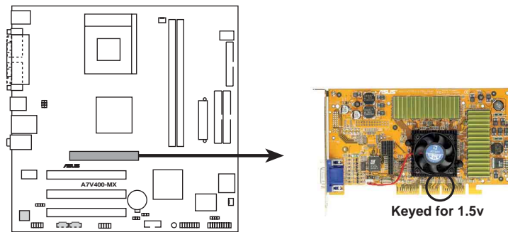
A7V400-MX Accelerated Graphics Port (AGP)
