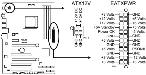
F2A55 ATX power connectors
