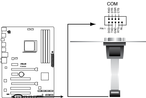
F2A55 Serial port (COM) connector
