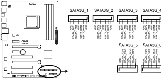
F2A55 SATA 3.0Gb/s connectors
