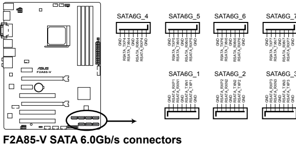
F2A85-V SATA 6.0Gb/s connectors
