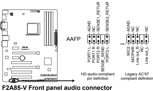
F2A85-V Front panel audio connector
