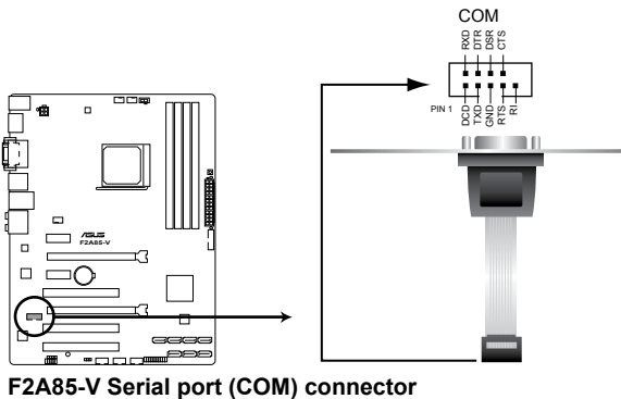
F2A85-V Serial port (COM) connector
