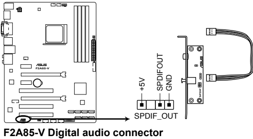
F2A85-V Digital audio connector
