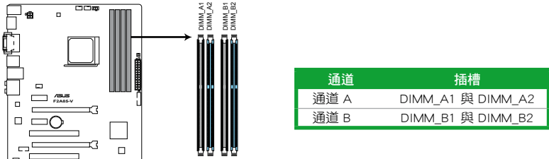
F2A85-V 240-pin DDR3 DIMM sockets
