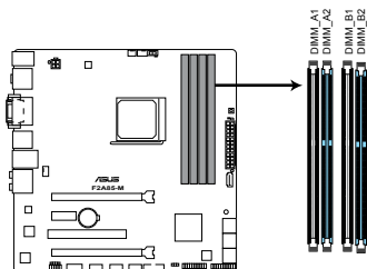
F2A85-M 240-pin DDR3 DIMM sockets
