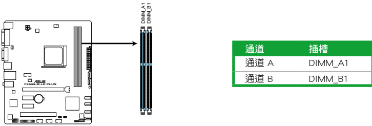
F2A55-M LK PLUS 240-pin DDR3 DIMM sockets
