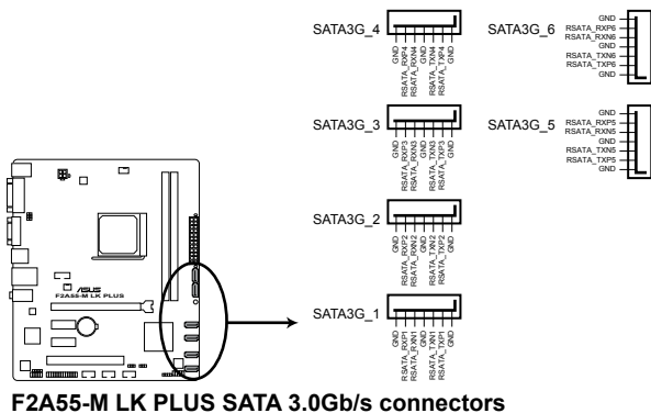
F2A55-M LK PLUS SATA 3.0Gb/s connectors
