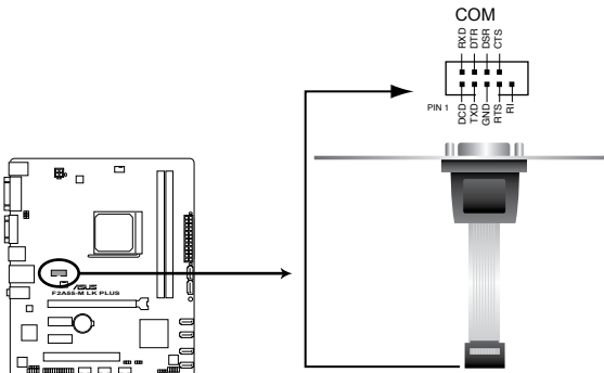
F2A55-M LK PLUS Serial port (COM) connector
