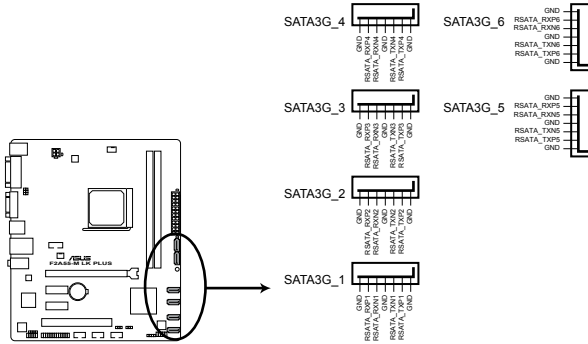
F2A55-M LK PLUS SATA 3.0Gb/s connectors
