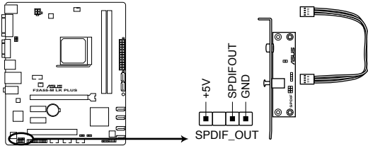
F2A55-M LK PLUS Digital audio connector
