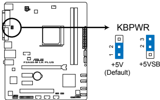
F2A55-M LK PLUS Keyboard power setting
