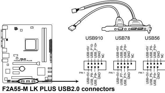
F2A55-M LK PLUS USB2.0 connectors
