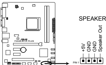
F2A55-M LK PLUS Speaker out connector
