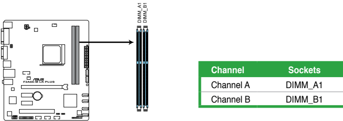
F2A55-M LK PLUS 240-pin DDR3 DIMM sockets
